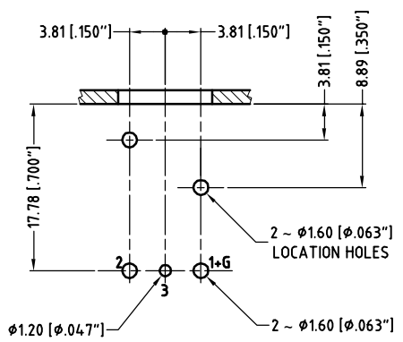
PCB - LAYOUT COMPONENT SIDE TOLERANCE: ±0.05mm [.002"]
