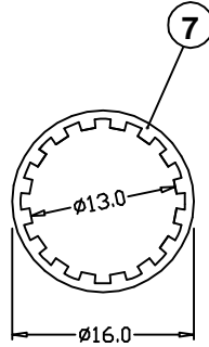
WASHER DETAIL
