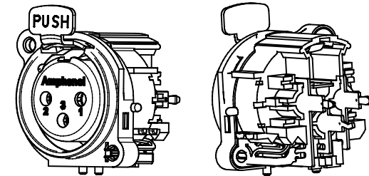
3D VIEW (1:1)
