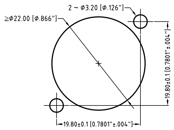
PANEL CUT OUT REAR VIEW
