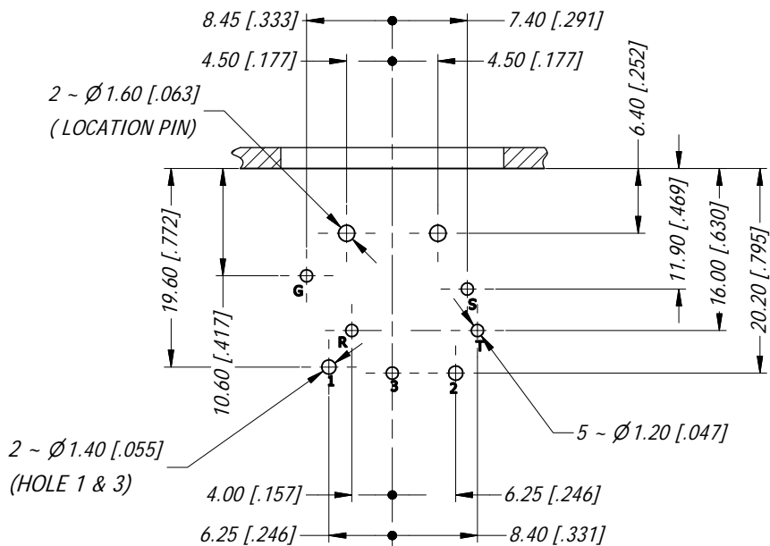
PCB LAYOUT SCALE 3:2
