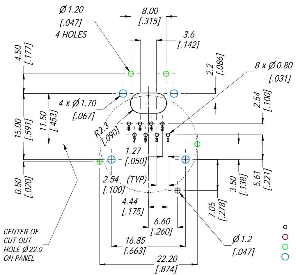
PCB LAYOUT 2:1 (CONNECTOR REAR VIEW)
