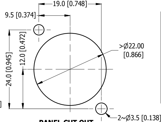
PANEL CUT OUT (SCALE 2:1)
