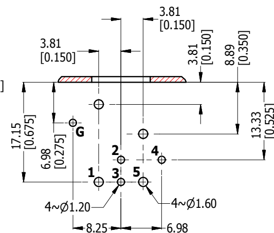
PCB LAYOUT COMPONENT SIDE TOLERANCE: ± 0.05mm [.002"]
