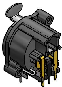
3D VIEW (1:1)
