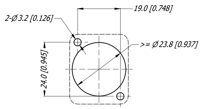
PANEL CUTOUT (1:1)
