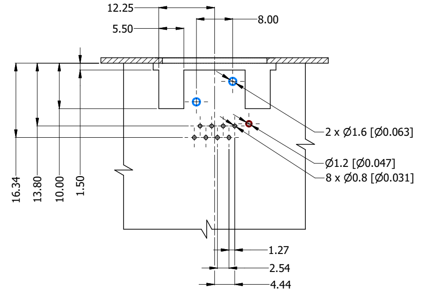
PCB LAYOUT (CONNECTOR TOP VIEW)
