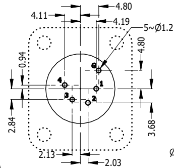
PCB LAYOUT CONNCTOR SIDE
