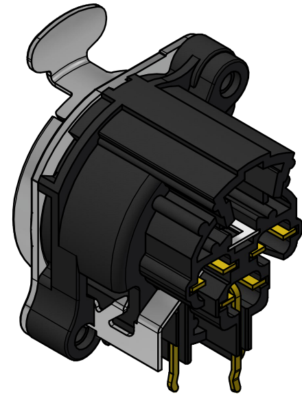
ISO VIEW
