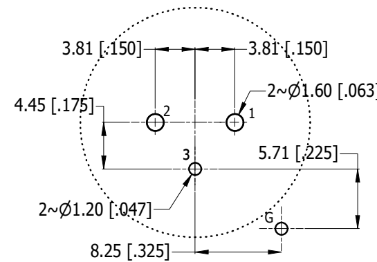
PCB-LAYOUT COMPONENT SIDE TOLERANCE: ±0.05mm [.002"]
