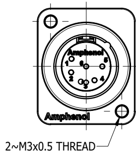
M3 THREAD OPTION
