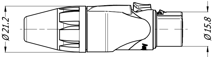
FEMALE CONNECTOR
