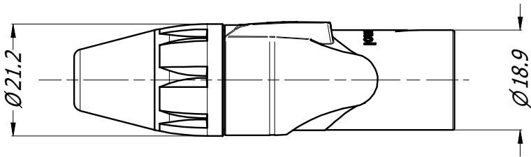
MALE CONNECTOR
