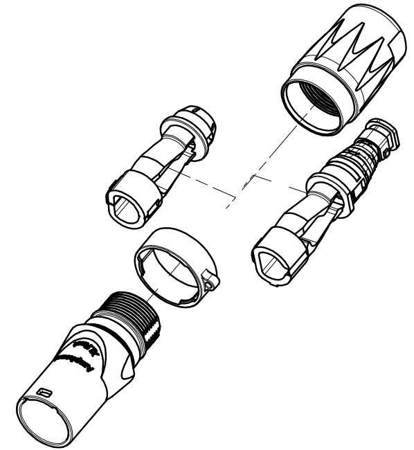
EXPLODED VIEW
