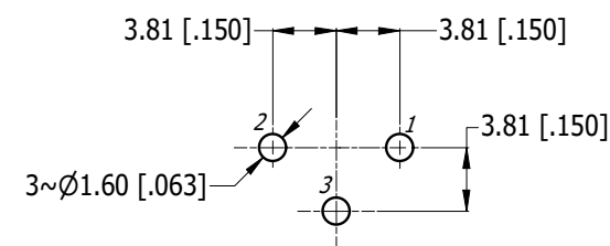
PCB-LAYOUT COMPONENT SIDE TOLERANCE: \pm 0.05\text{mm} [0.002"]
