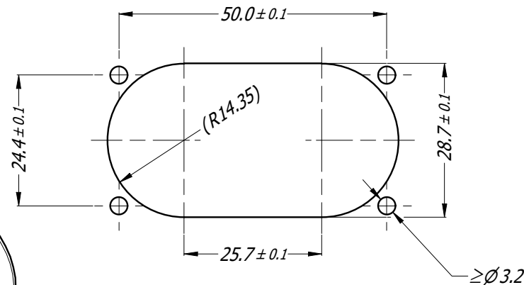
PANEL CUTOUT
