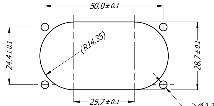
PANEL CUTOUT
