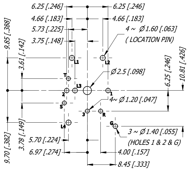
PCB LAYOUT SCALE 3:2
