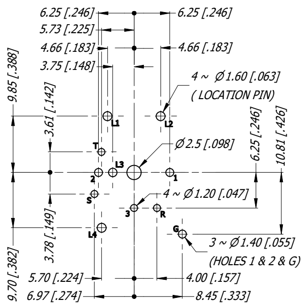
PCB LAYOUT SCALE 3:2
