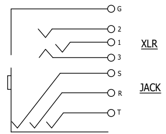
CONTACT SCHEMATIC DIAGRAM
